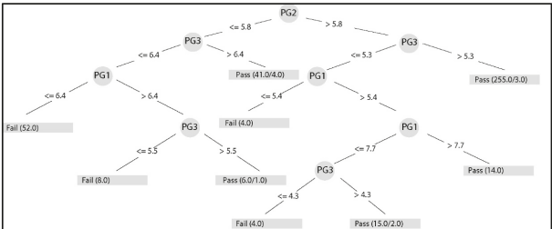
Figure 12. Decision tree to predict the results of the students in the last year.
