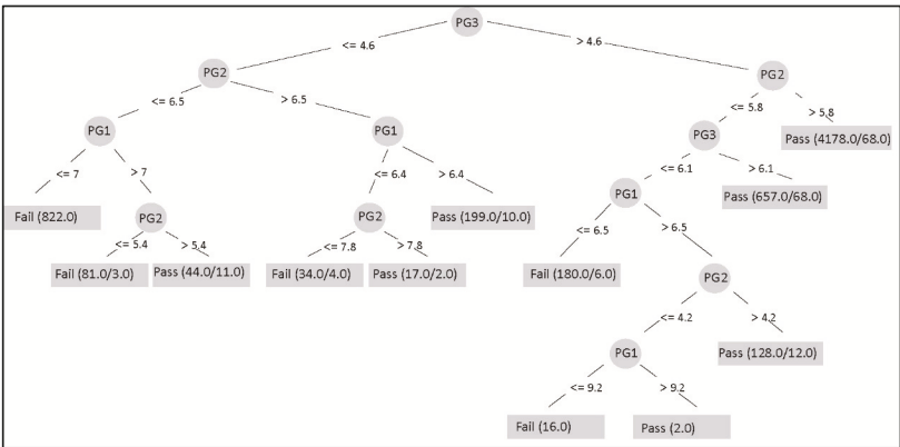
Figure 9. Decision tree without the FG.
