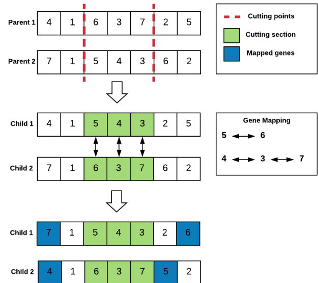
FIGURE 9. Partially mapped crossover.
